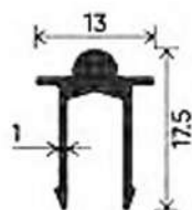
TRACK RAIL CLIP
