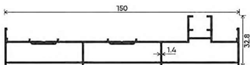
THREE TRACK SIDE
