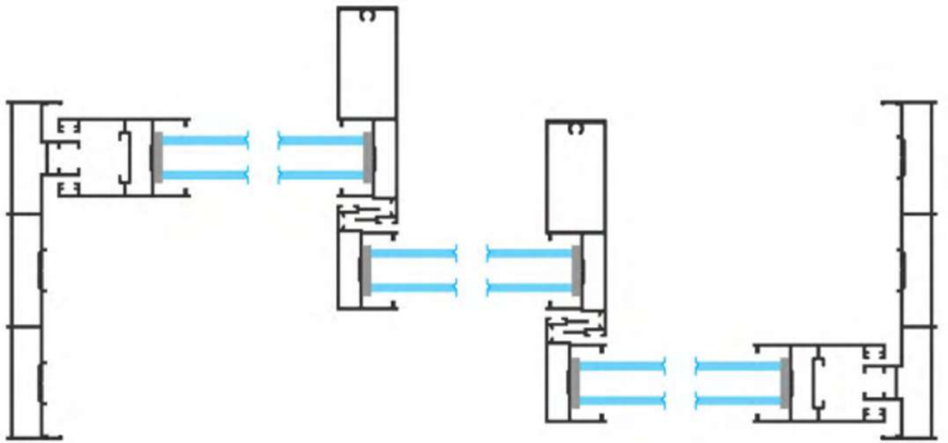
Top View
