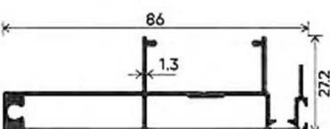
SHUTTER
