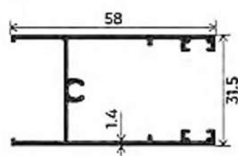
SHUTTER
