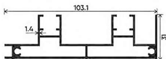
TRACK
