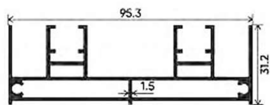
TWO TRACK
