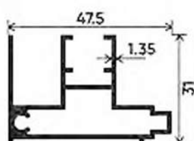
TRACK
