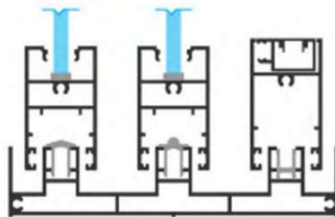
Three Track with Mosquito Assamble
