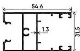
SHUTTER
