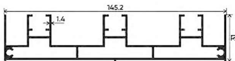
THREE TRACK
