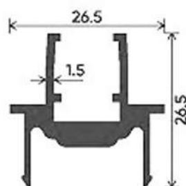
MEETING SECTION
