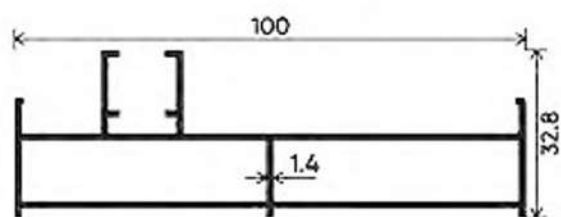
TWO TRACK SIDE
