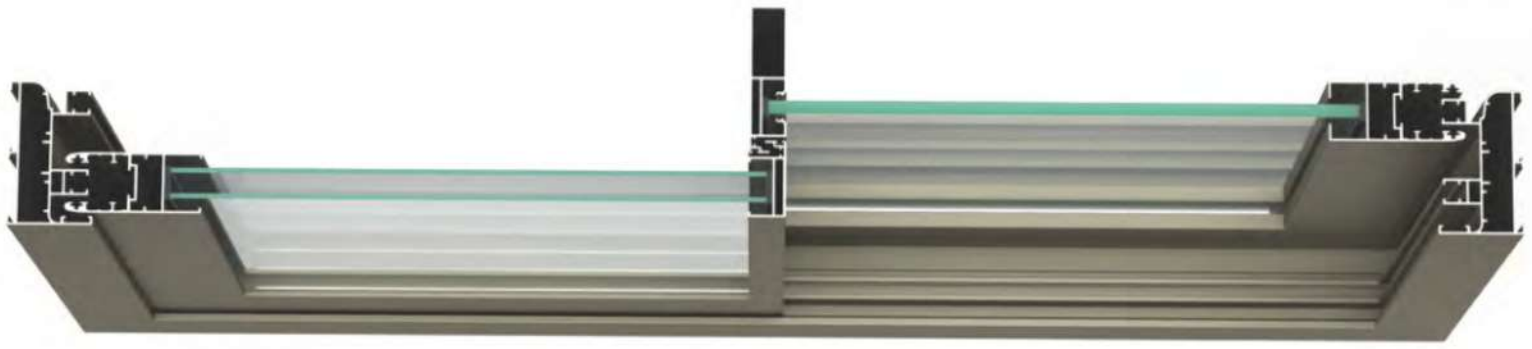
Top View
