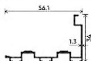
SHUTTER CLIP
