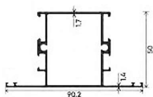
MULLION
