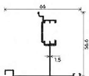
MULLION
