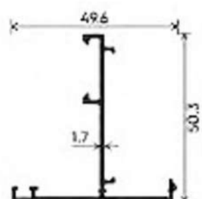
ADAPTER
