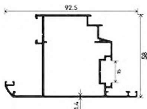
SHUTTER
