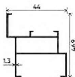
FRAME
