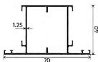
SHUTTER
