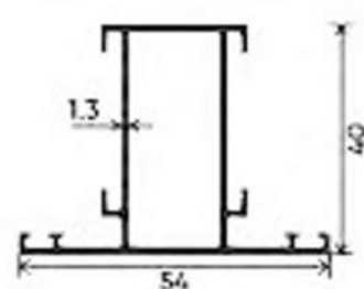
ECO MULLION
