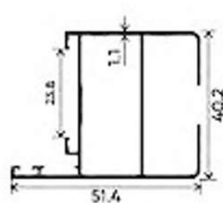
MIDDLE SECTION
