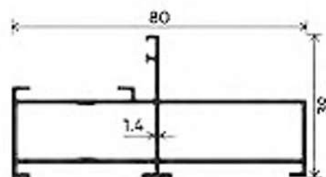
FRAME
