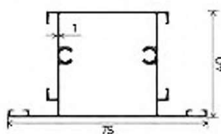
SHUTTER
