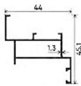
SHUTTER
