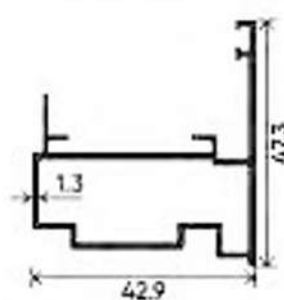
FLY MULLION
