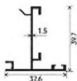
ADAPTOR
