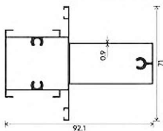
KPA MULLION
