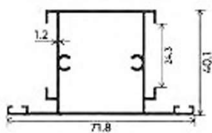
SHUTTER
