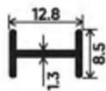
GLASS JOINT
