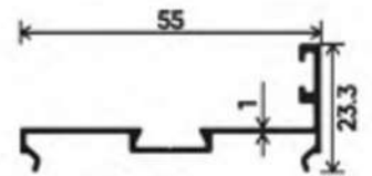
DOOR COVER FOR FIXED PROFILE
