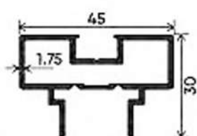
HORIZONTAL PROFILE
