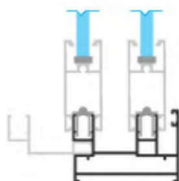
Top & Bottom Shutter
