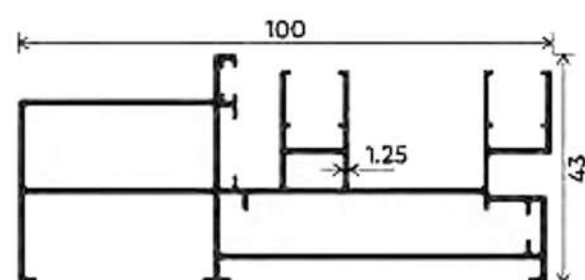
TWO TRACK
