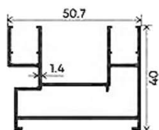
TWO TRACK
