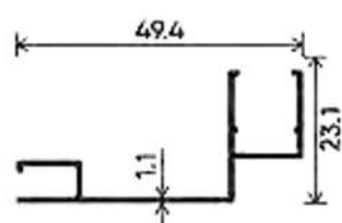
ADDITIONAL TRACK
