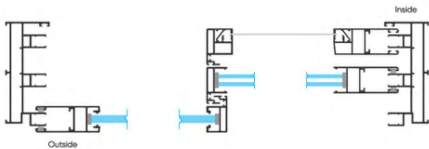
Top View
