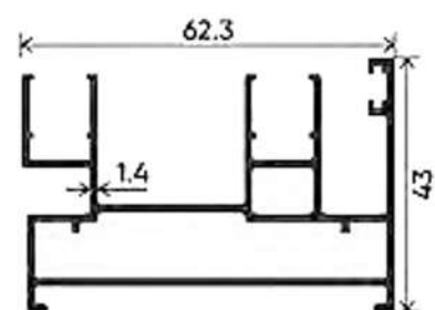
TWO TRACK
