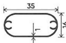
GRILL SUPPORT
