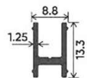
TRACK RAIL CAP
