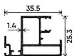
SHUTTER
