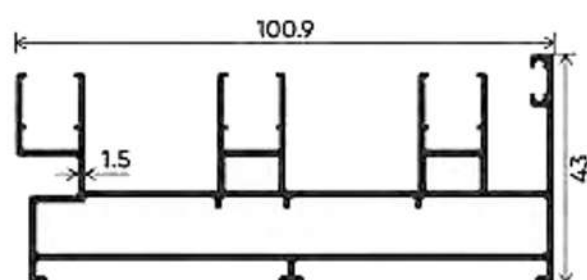
THREE TRACK
