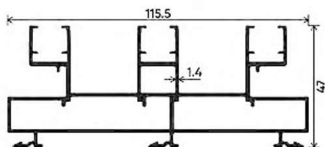
THREE TRACK
