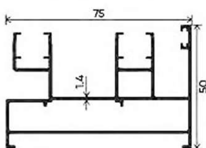
TWO TRACK
