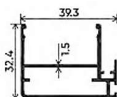
SHUTTER
