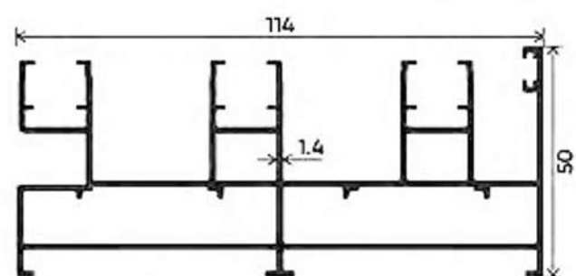
THREE TRACK
