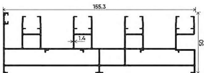
FOUR TRACK
