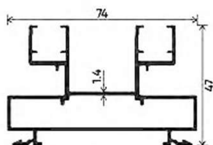
TWO TRACK
