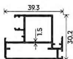
SHUTTER
