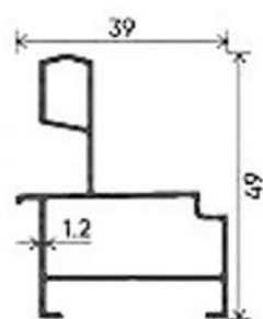
ADDITIONAL TRACK
