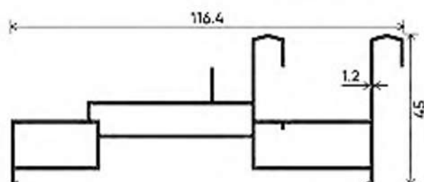
TWO TRACK
