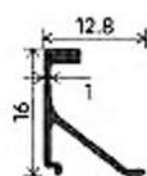
SHUTTER CLIP
