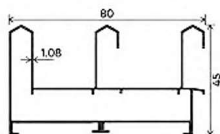
THREE TRACK
