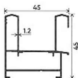
TWO TRACK
