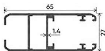
SHUTTER
