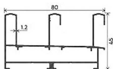
THREE TRACK
