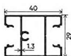
SHUTTER
