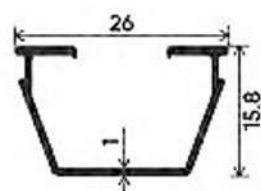
REDUCER CLIP
