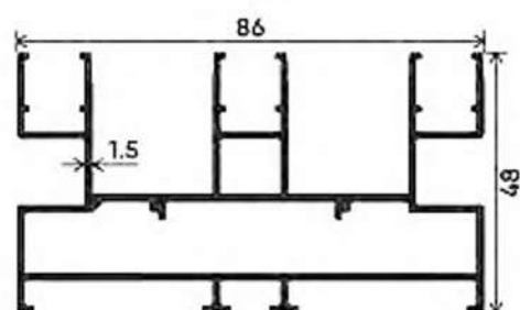
THREE TRACK
