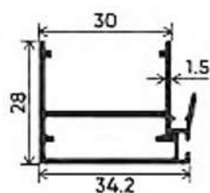
SHUTTER
