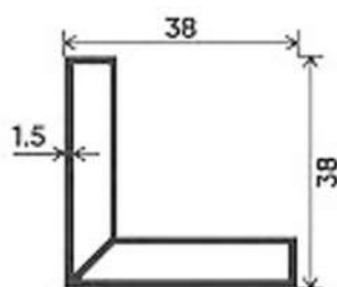
ANGLE
