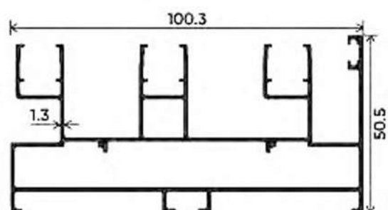
THREE TRACK
