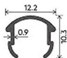
MOSQUITO CLIP
