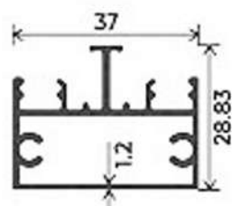
MIDDLE SHUTTER
