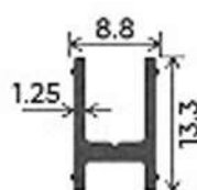
TRACK RAIL CAP
