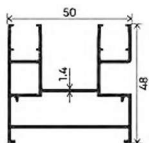
TWO TRACK
