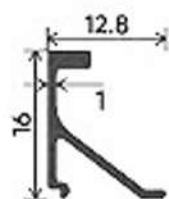
SHUTTER CLIP
