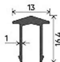
TRACK RAIL CLIP
