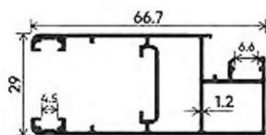
SHUTTER
