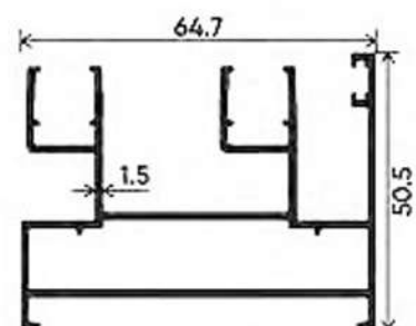
TWO TRACK
