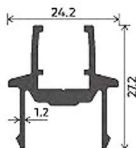
MEETING SECTION
